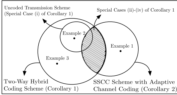
General JSCC Scheme (Theorem 1)
